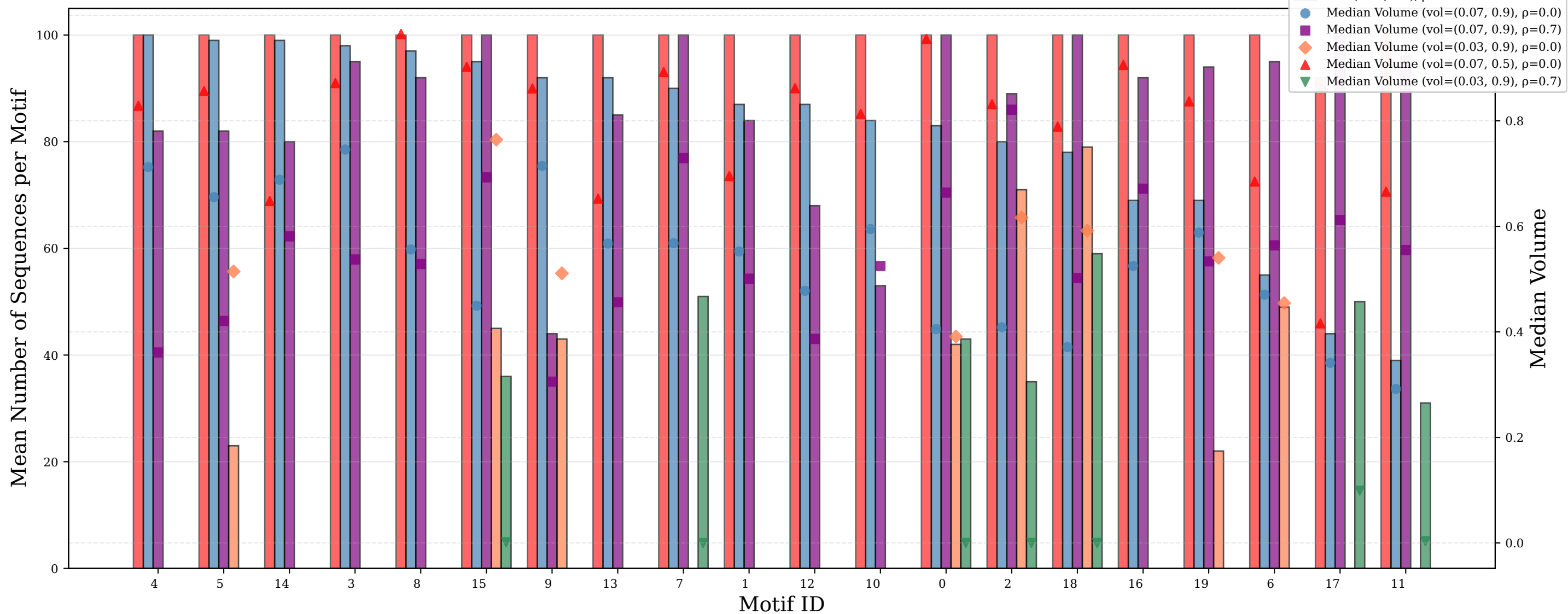
Number of Sequences per Motif & Median Volume at R=100 for Different Volume Parameters and Correlations sigma=(0.02, 0.4)
